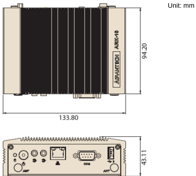
Figure 1.1 ARK-10 mechanical dimension drawing
