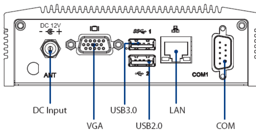
Figure 2.1 ARK-10 I/O view
