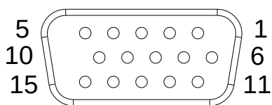
Figure 2.5 VGA Connector
