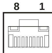
Figure 2.4 Ethernet Connector
