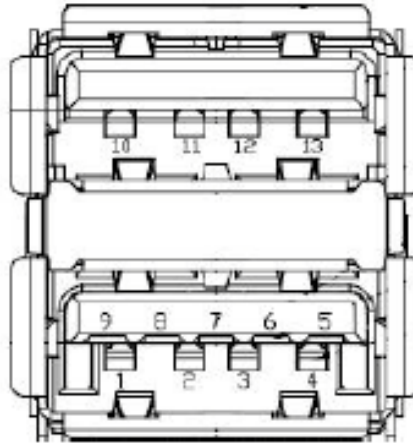
Figure 2.6 USB Connector
