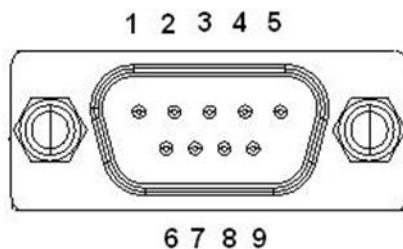
Figure 2.8 COM Port Connector
